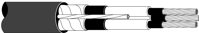
Three-Conductor Non-Armored, Shielded Cable
