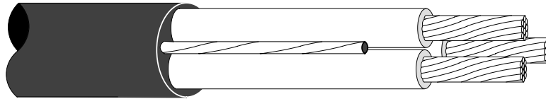
Three-Conductor Non-Armored, Nonshielded Cable
